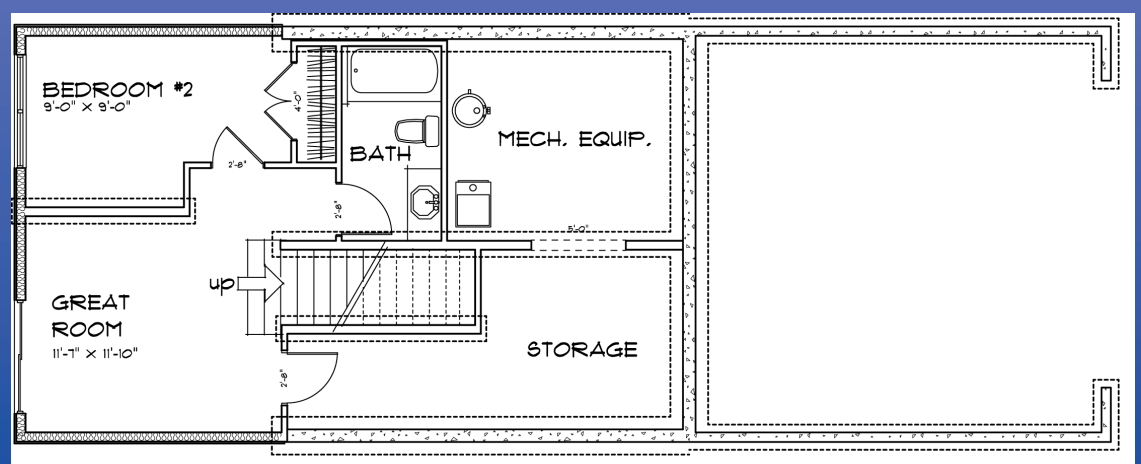
LOWER LEVEL FLOOR PLAN
